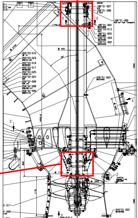
Kaplan Hydro Turbine Diagram
